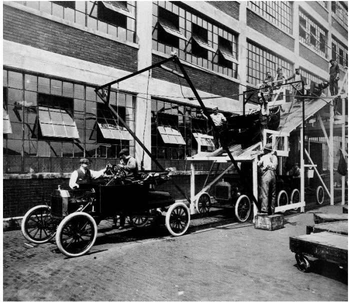
An outdoor line for the Model T, circa 1914. The carbody is dropped from a ramp on to the chassis. (A History of Ford Motor Company, 1992, p.24.)
